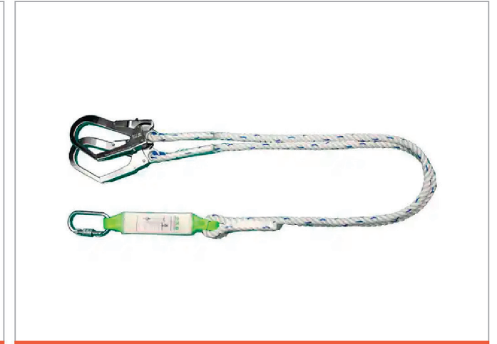
FBO-TE6114 Energy absorber lanyards Rope:1.3-2m Bearing:2.2 tons Energy absorber lanyards: 0.75m
